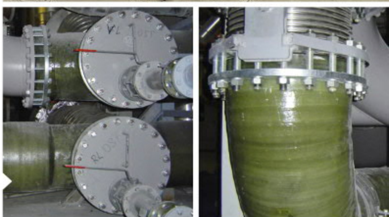
Cooling water system DN3600
